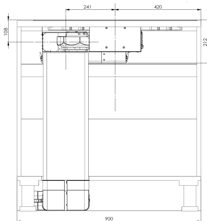
Rear view of 90 cm cabinet
