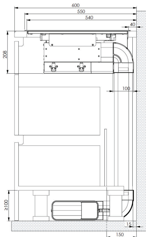
Side view in built-in condition
